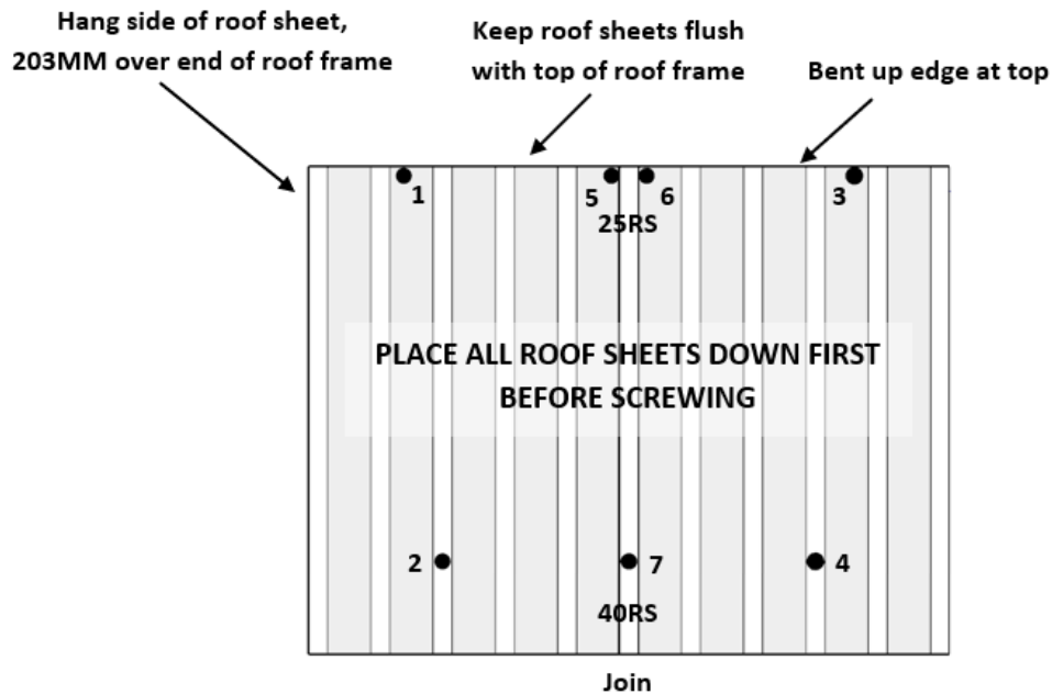
(SIDE VIEW)
